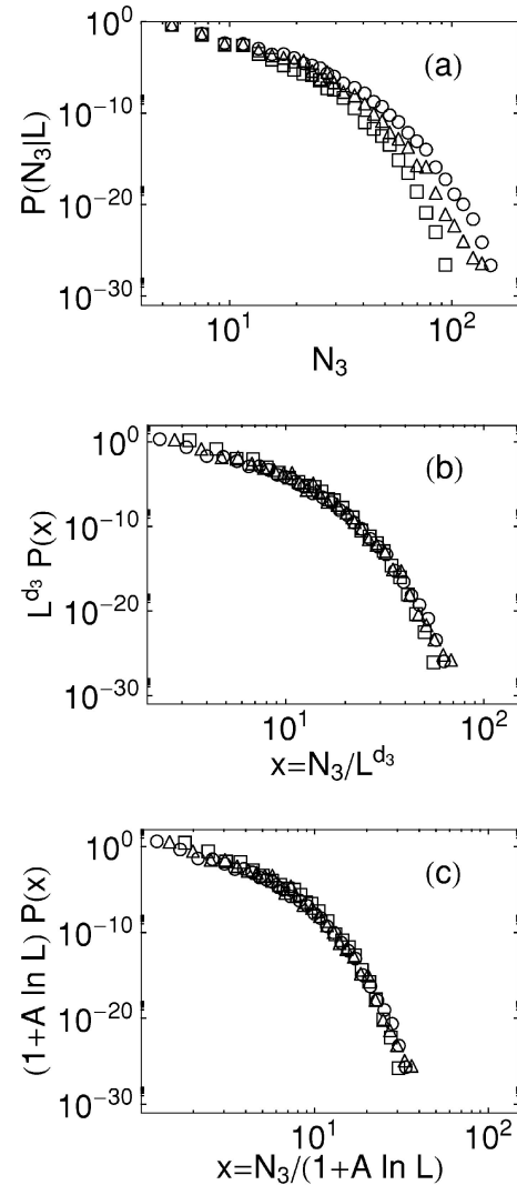
FIG. 4. P(N_3|L) , the distribution of 3-block mass N_3 for (from left to right) L=8, 16, and 32 for the case of six dimensions. (a) uncollapsed, (b) collapsed using a value of d_3=0.25 , (c) collapsed assuming N_3 \sim 1 + A \ln L with A=1.0 .
