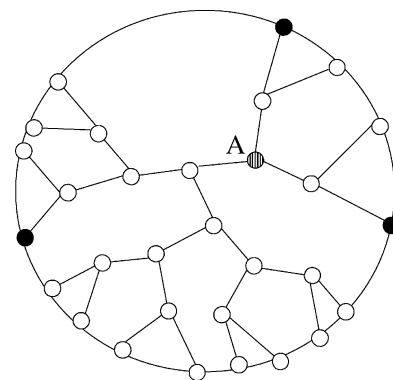
FIG. 1. Cayley tree in which each site except those on boundary has three neighbors. We note that even when all bonds are fully occupied, there can be only one site which is connected to three sites on the boundary. In this example the three sites on the boundary are the filled circles and the one site connected to them by independent paths is the striped circle denoted by A.
