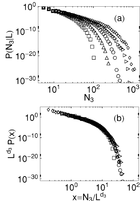
FIG. 2. P(N_3|L) , the distribution of 3-block mass N_3 for (from left to right) L=8, 16, 32, 64, and 128 for the case of four dimensions. (a) uncollapsed, (b) collapsed using a value of d_3=0.7 .
